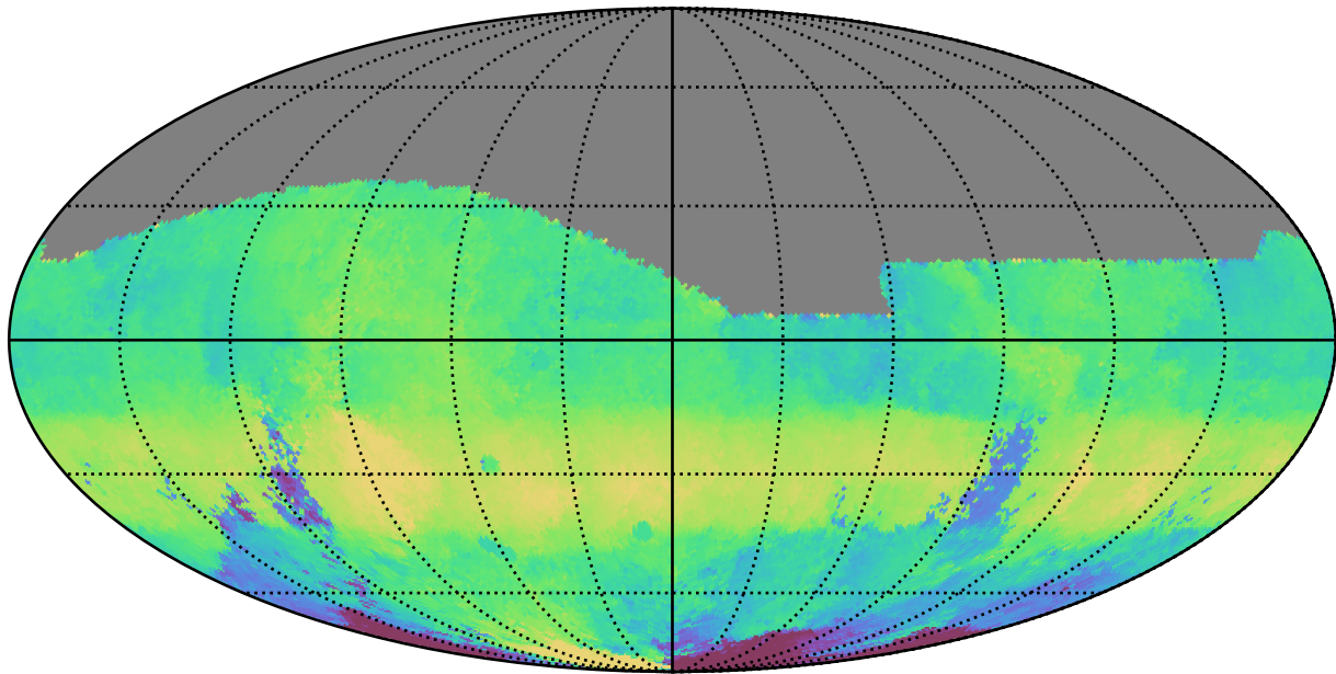
ddf_acor_sf10_lsf15_lsr10_v3.4_10yrs All sky g band: Median HA
