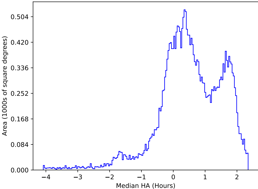
ddf_acor_sf10_ls15_lsr10_v3.4_10yrs All sky g band: Median HA
