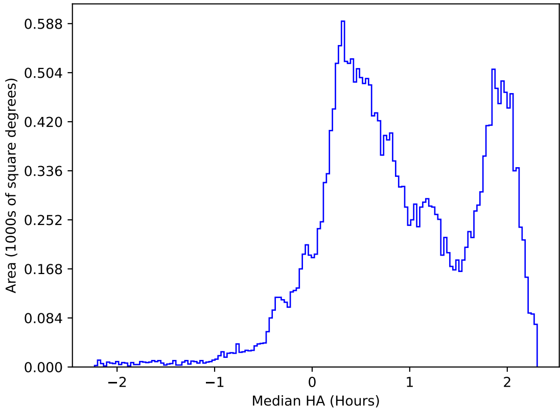
ddf_acor_sf10_lsf15_lsr10_v3.4_10yrs All sky all bands: Median HA
