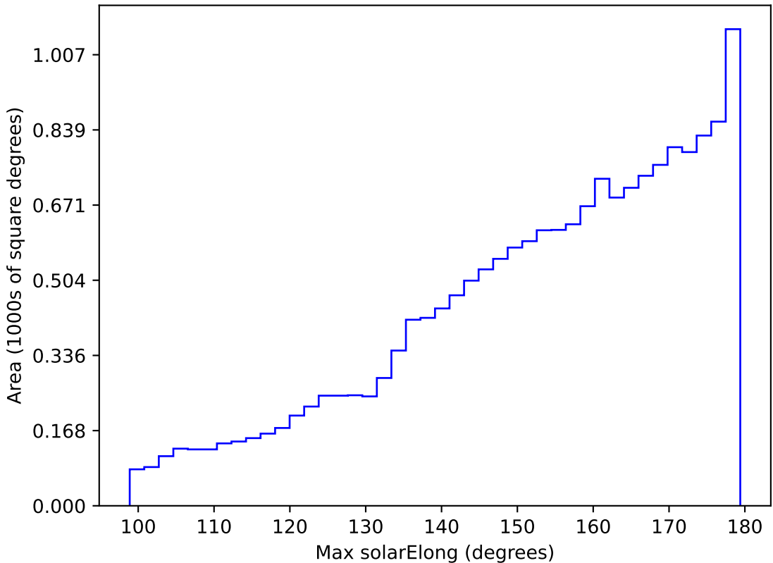
ddf_acor_sf10_lsf15_lsr10_v3.4_10yrs WFD z band: Max solarElong
