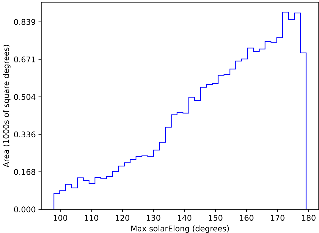
ddf_acor_sf10_lsf15_lsr10_v3.4_10yrs WFD u band: Max solarElong
