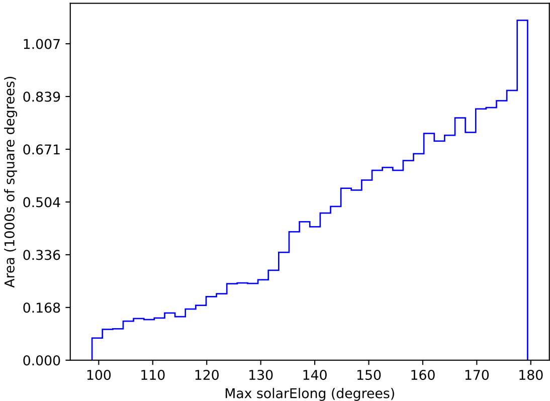
ddf_acor_sf10_lsf15_lsr10_v3.4_10yrs WFD r band: Max solarElong
