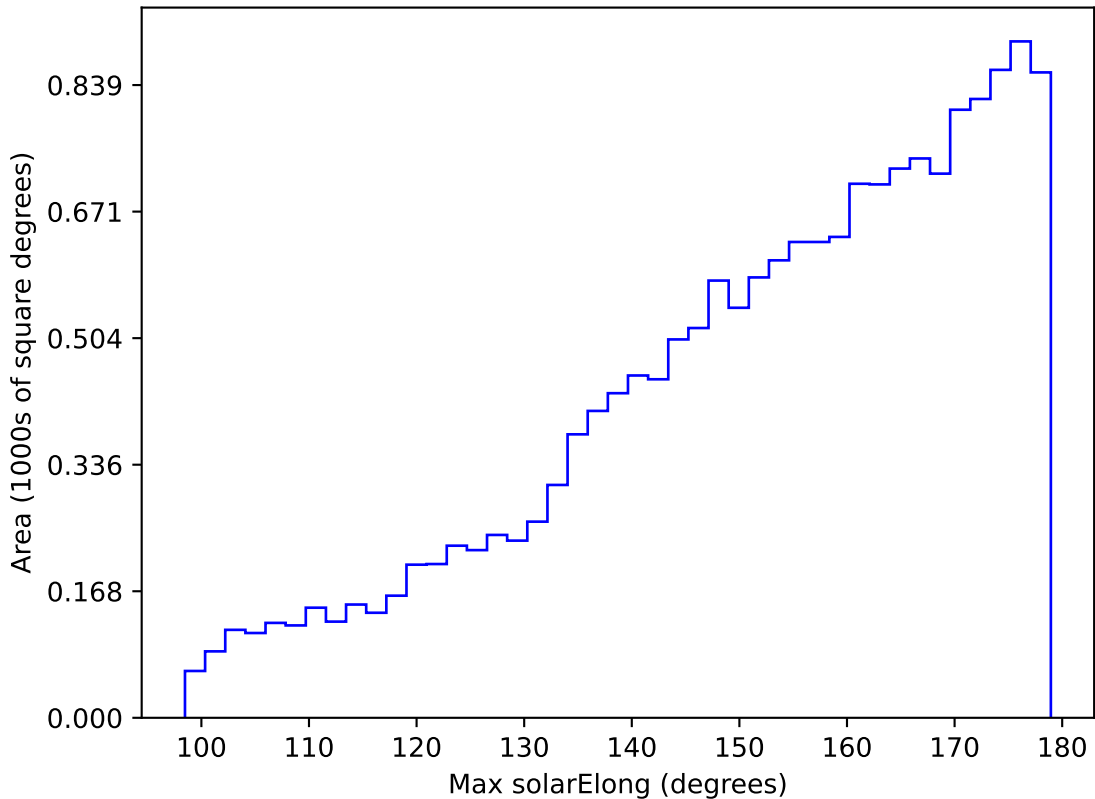
ddf_acor_sf10_lsf15_lsr10_v3.4_10yrs WFD g band: Max solarElong
