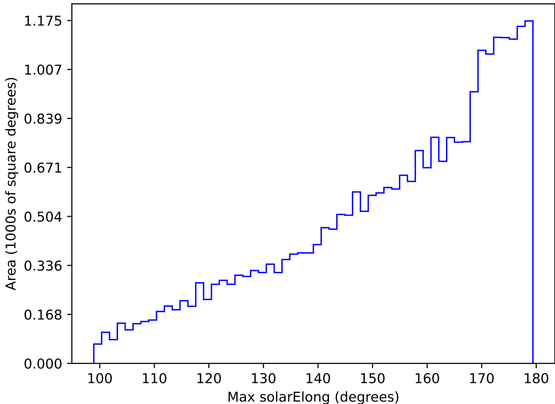
ddf_acor_sf10_lsf15_lsr10_v3.4_10yrs All sky z band: Max solarElong
