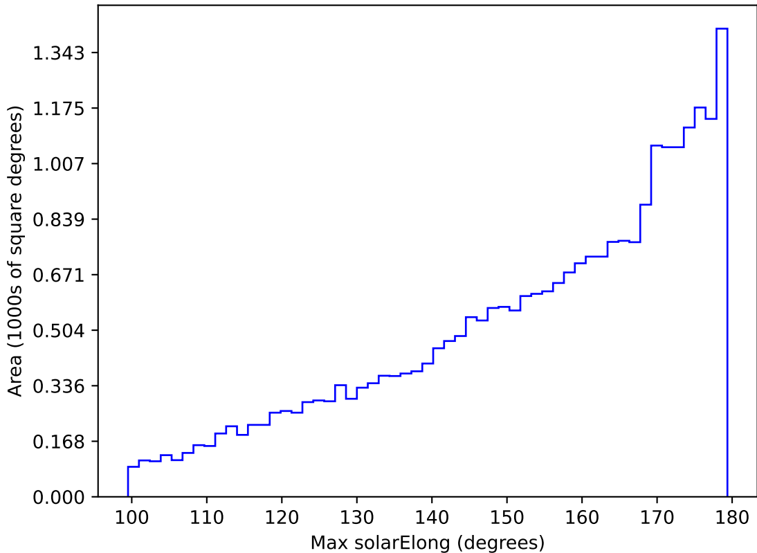
ddf_acor_sf10_lsf15_lsr10_v3.4_10yrs All sky r band: Max solarElong
