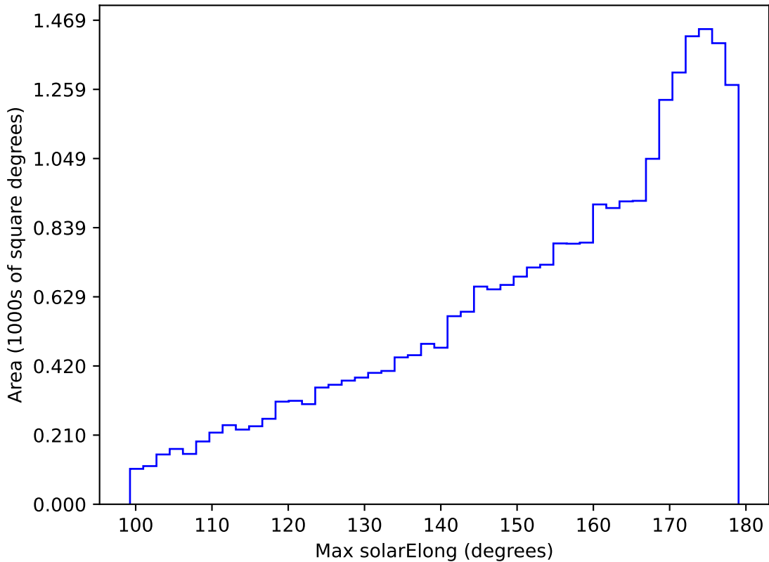
ddf_acor_sf10_lsf15_lsr10_v3.4_10yrs All sky g band: Max solarElong
