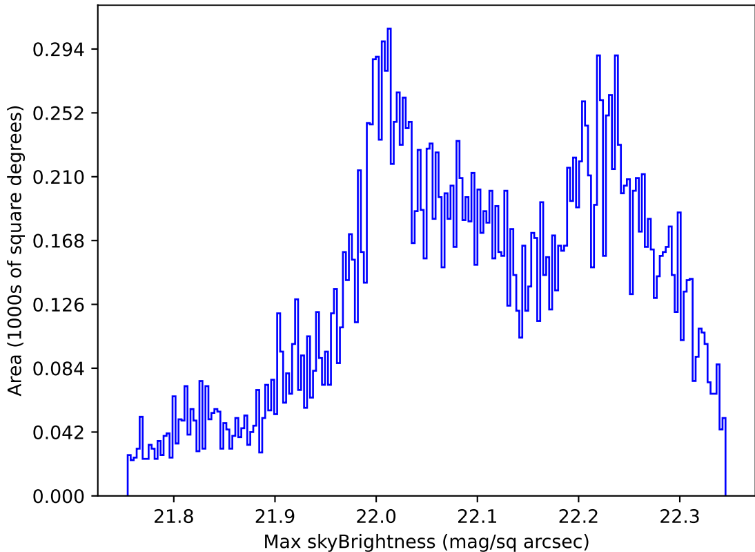
ddf_acor_sf10_lsf15_lsr10_v3.4_10yrs Yr 1 g band: Max skyBrightness
