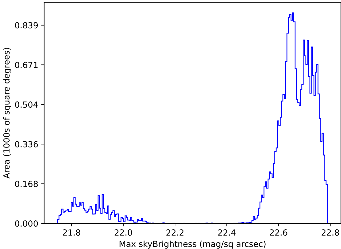
ddf_acor_sf10_lsf15_lsr10_v3.4_10yrs Yr 1 all bands: Max skyBrightness
