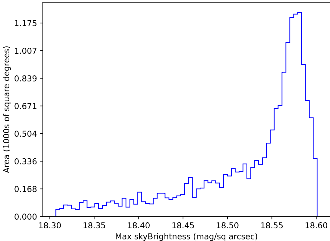
ddf_acor_sf10_lsf15_lsr10_v3.4_10yrs WFD y band: Max skyBrightness
