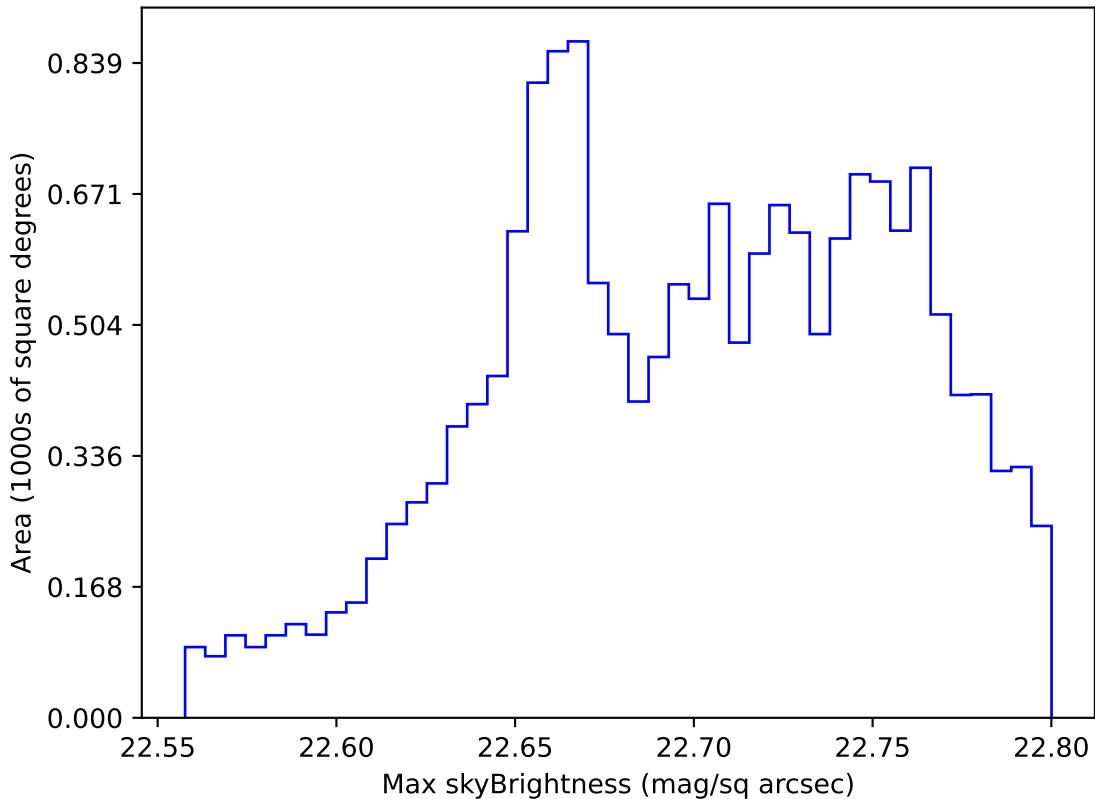
ddf_acor_sf10_lsf15_lsr10_v3.4_10yrs WFD u band: Max skyBrightness
