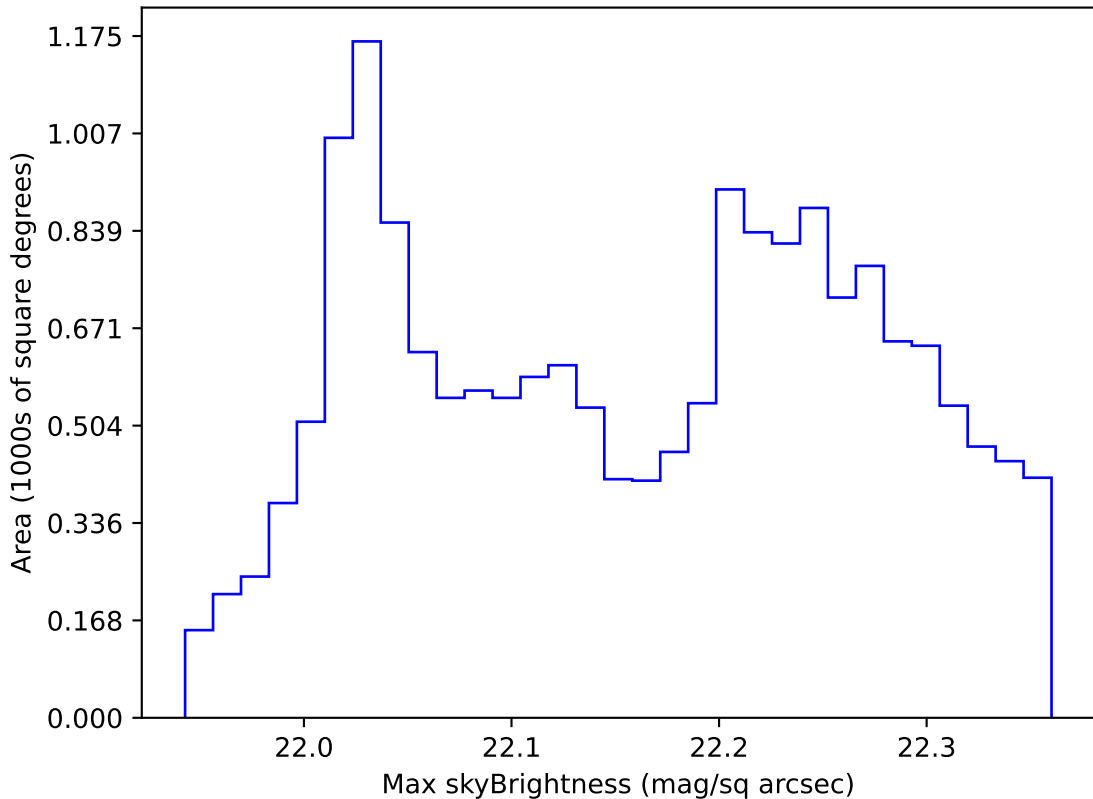
ddf_acor_sf10_lsf15_lsr10_v3.4_10yrs WFD g band: Max skyBrightness
