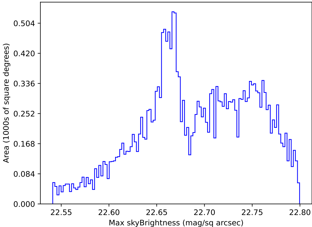
ddf_acor_sf10_lsf15_lsr10_v3.4_10yrs All sky u band: Max skyBrightness
