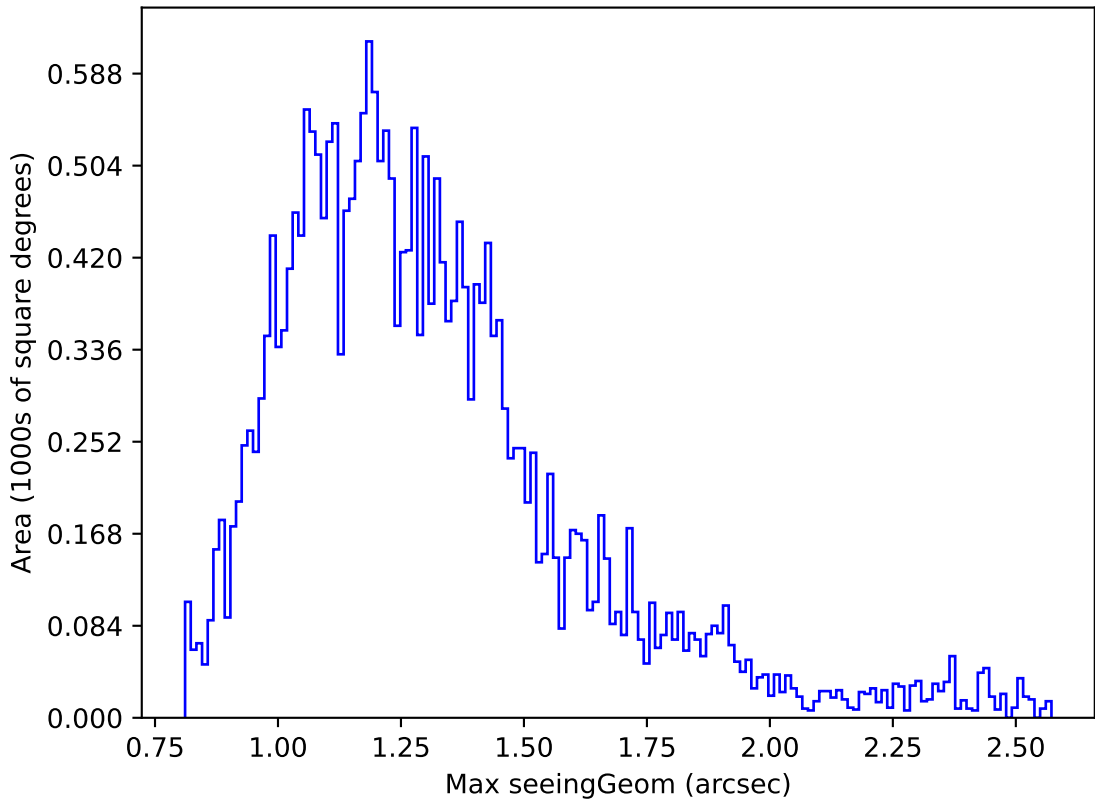
ddf_acor_sf10_lsf15_lsr10_v3.4_10yrs Yr 1 z band: Max seeingGeom
