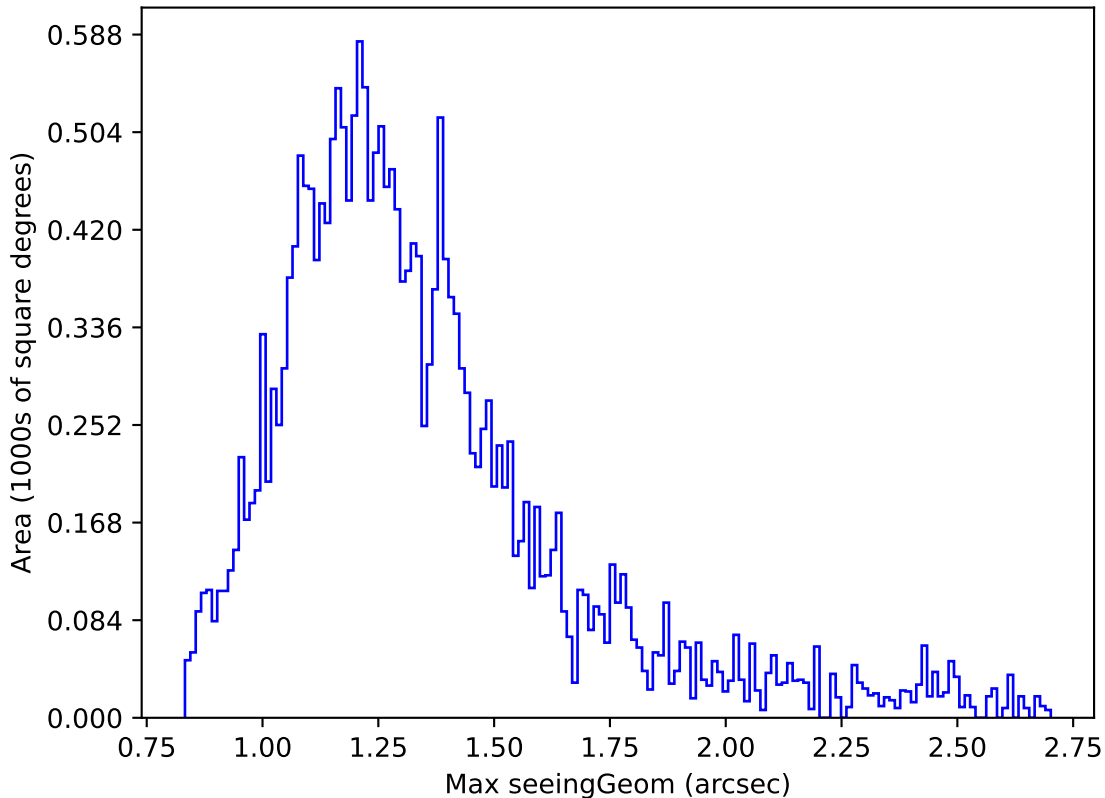
ddf_acor_sf10_lsf15_lsr10_v3.4_10yrs Yr 1 u band: Max seeingGeom
