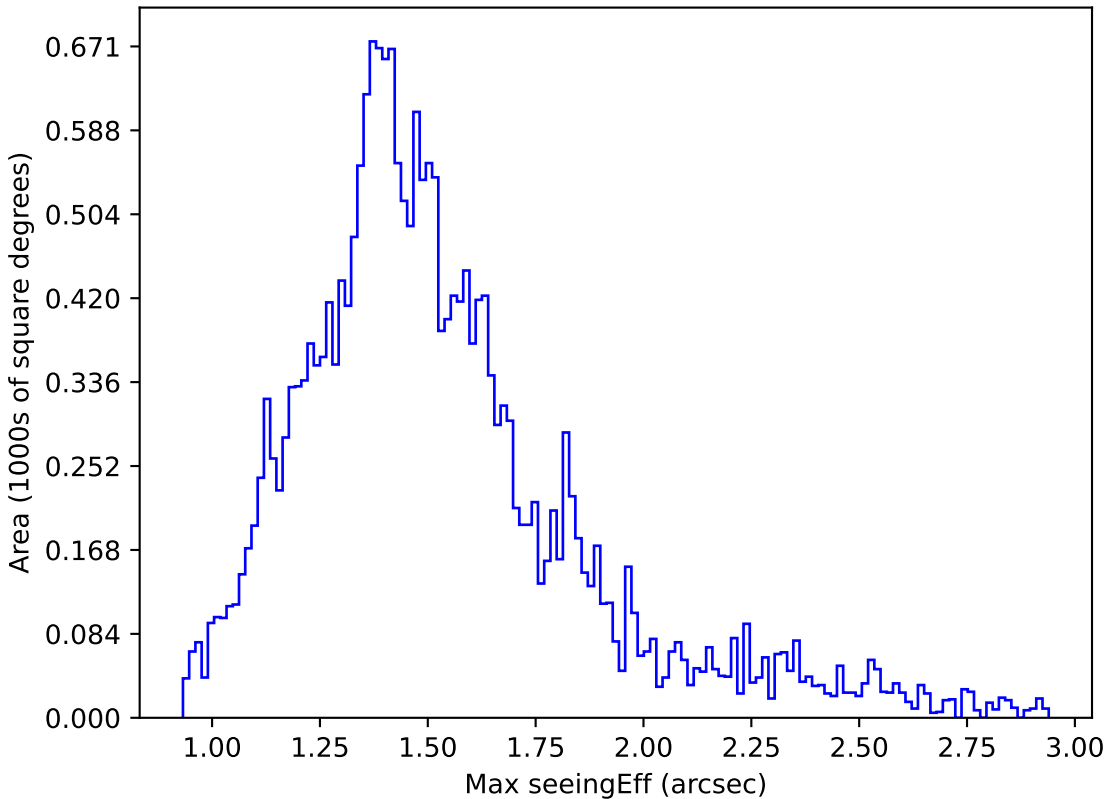
ddf_acor_sf10_lsf15_lsr10_v3.4_10yrs Yr 1 y band: Max seeingEff
