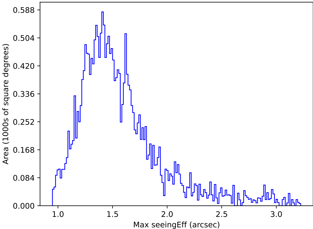
ddf_acor_sf10_lsf15_lsr10_v3.4_10yrs Yr 1 u band: Max seeingEff
