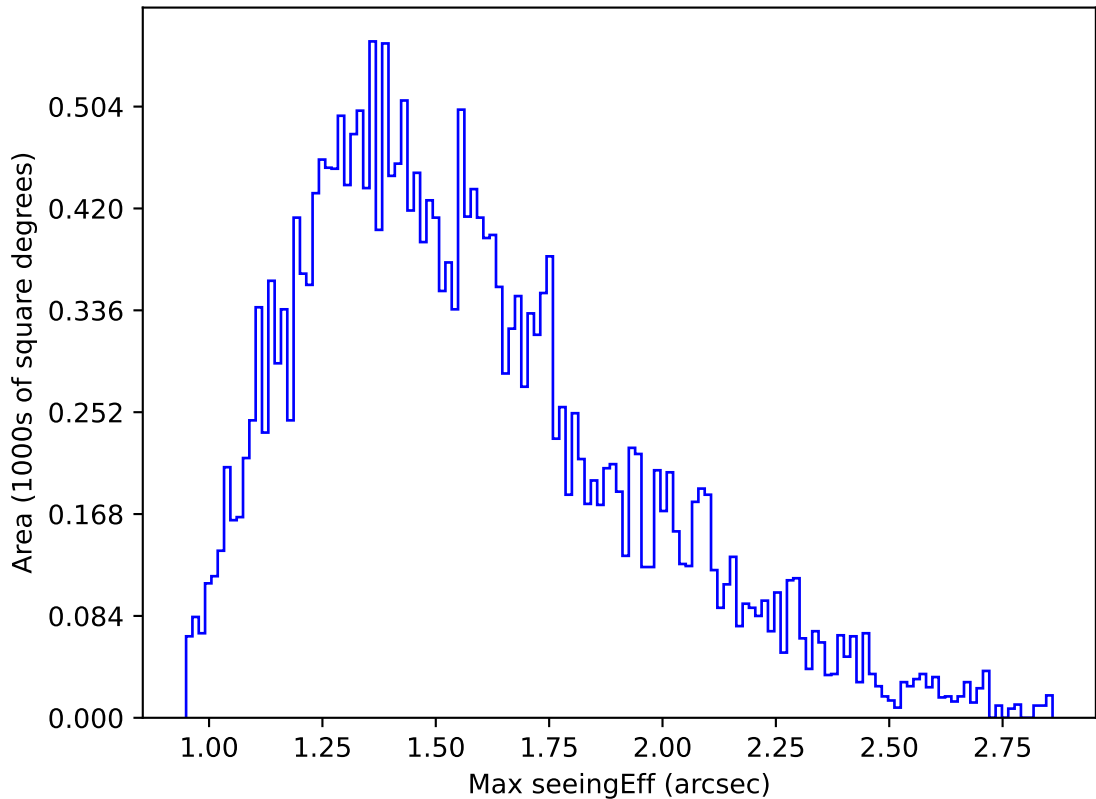
ddf_acor_sf10_lsf15_lsr10_v3.4_10yrs Yr 1 r band: Max seeingEff
