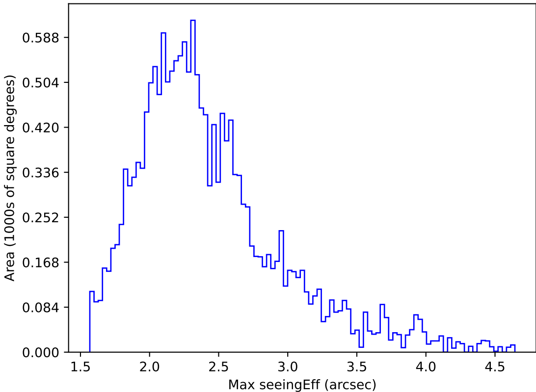
ddf_acor_sf10_lsf15_lsr10_v3.4_10yrs WFD y band: Max seeingEff
