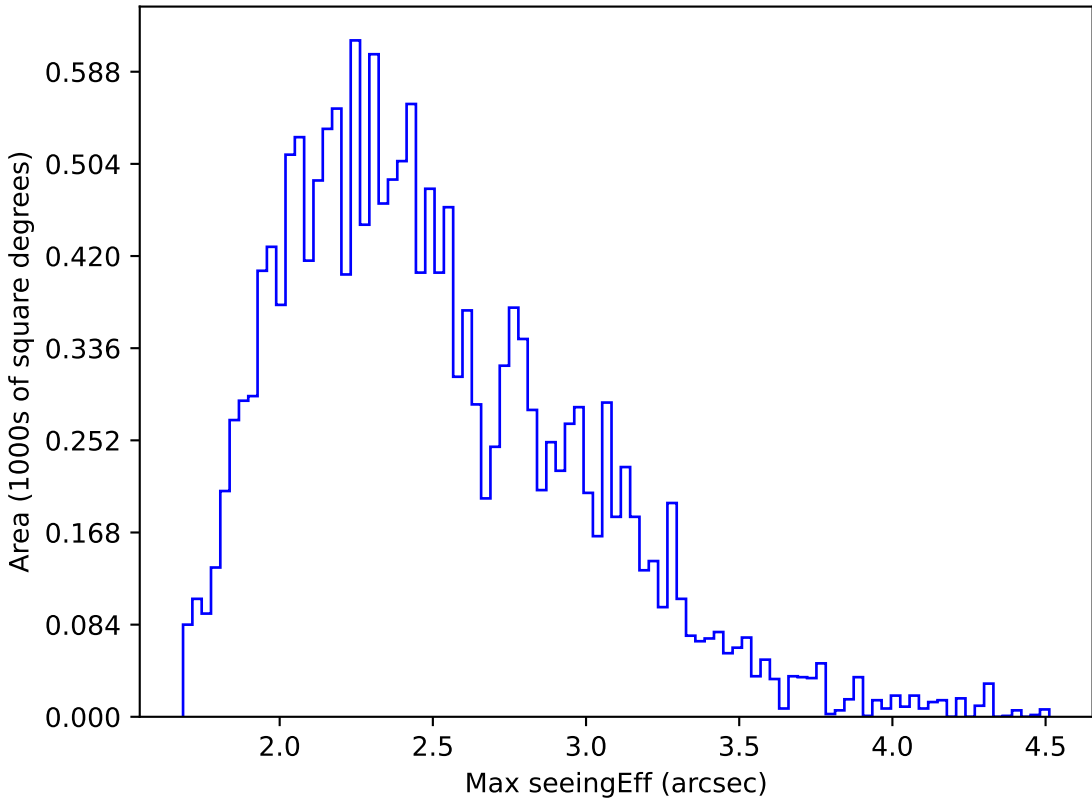
ddf_acor_sf10_lsf15_lsr10_v3.4_10yrs WFD u band: Max seeingEff
