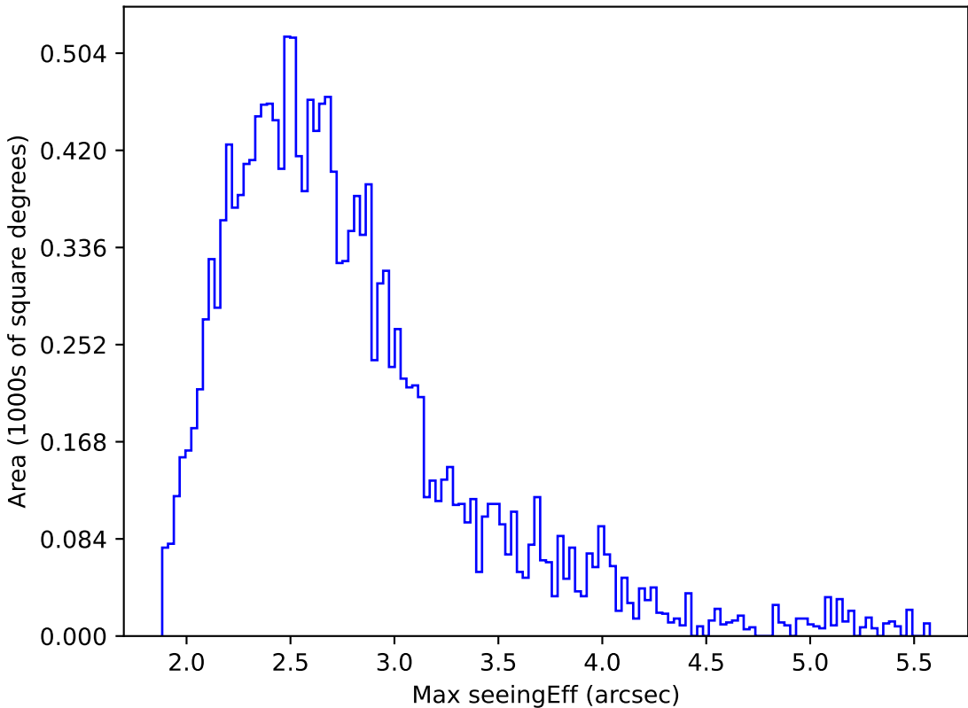
ddf_acor_sf10_lsf15_lsr10_v3.4_10yrs WFD r band: Max seeingEff
