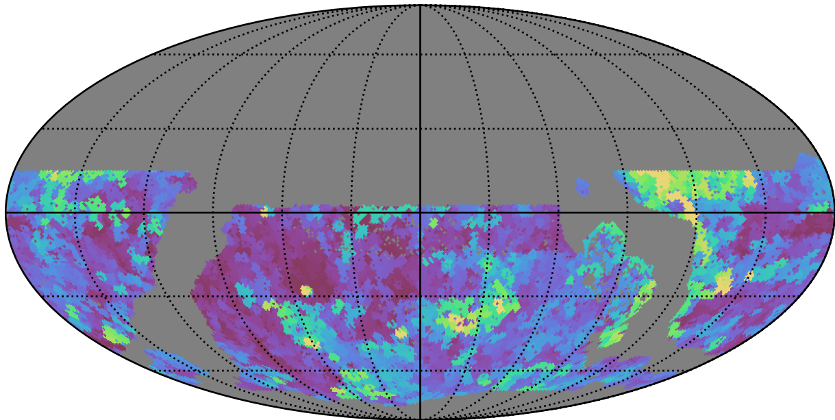
ddf_acor_sf10_lsf15_lsr10_v3.4_10yrs WFD g band: Max seeingEff
