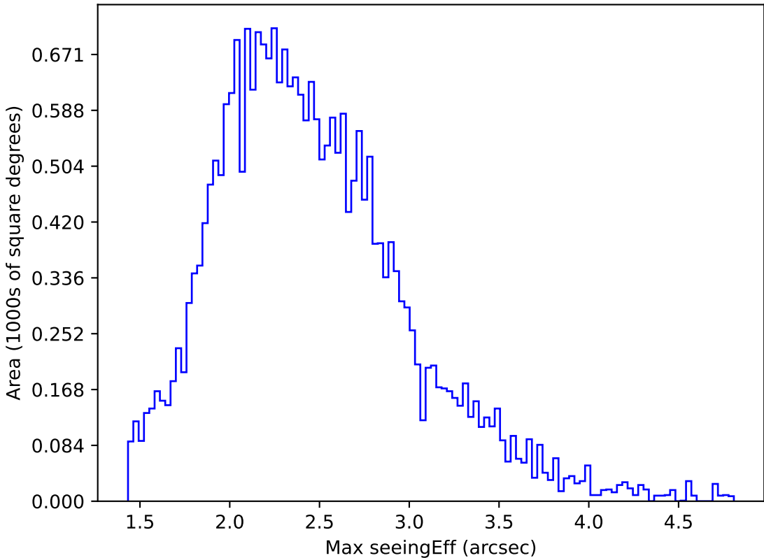
ddf_acor_sf10_lsf15_lsr10_v3.4_10yrs All sky z band: Max seeingEff
