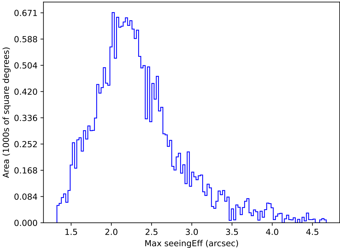
ddf_acor_sf10_ls15_lsr10_v3.4_10yrs All sky y band: Max seeingEff
