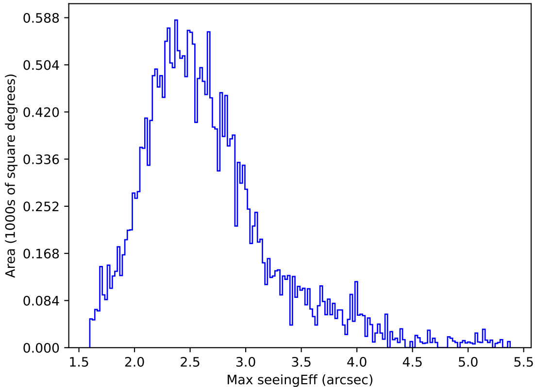
ddf_acor_sf10_lsf15_lsr10_v3.4_10yrs All sky r band: Max seeingEff
