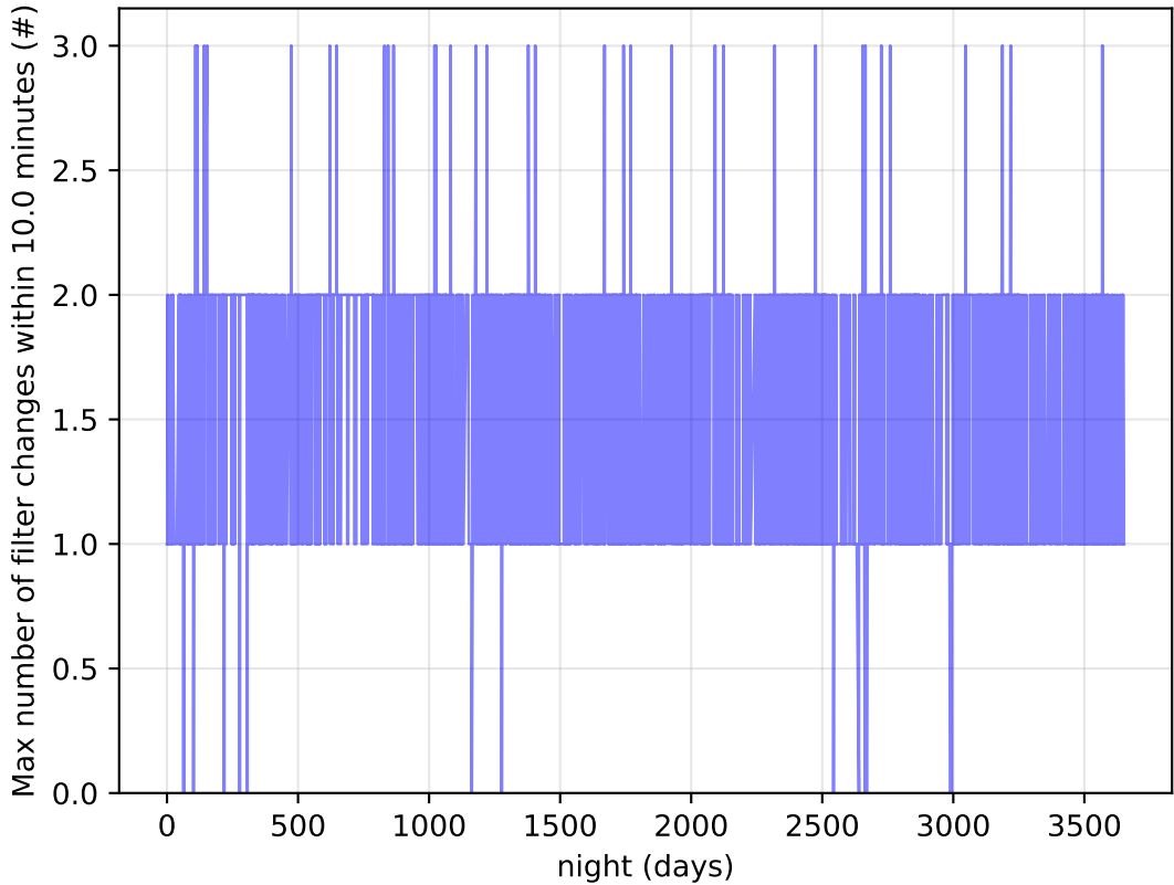
ddf_acor_sf10_Isf15_Isr10_v3.4_10yrs Per Night: Max number of filter changes within 10.0 minutes
