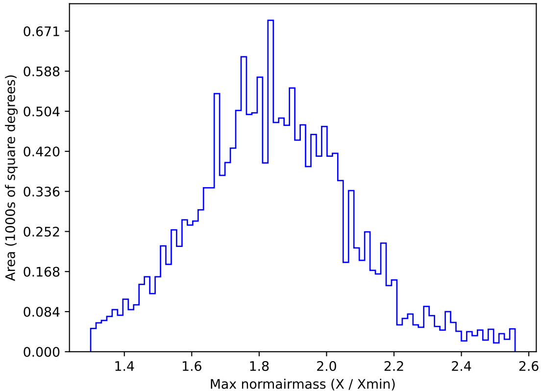
ddf_acor_sf10_lsf15_lsr10_v3.4_10yrs WFD g band: Max normairmass
