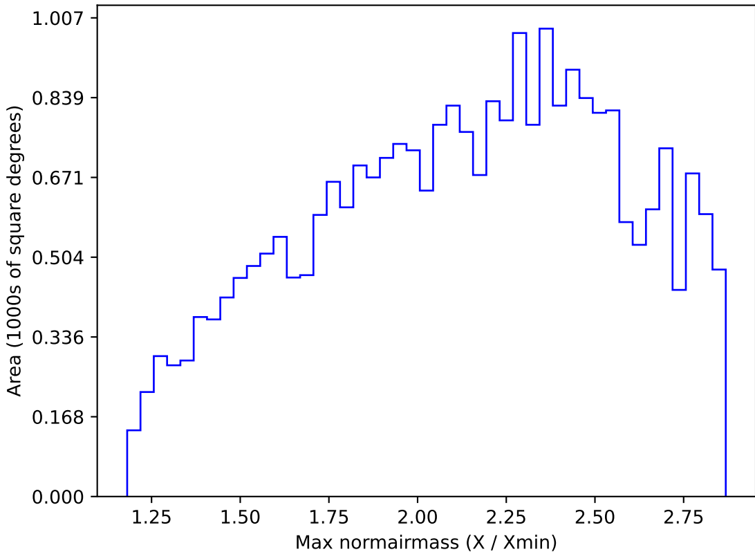
ddf_acor_sf10_lsf15_lsr10_v3.4_10yrs All sky i band: Max normairmass
