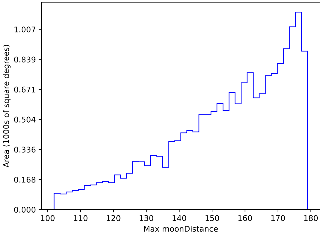
ddf_acor_sf10_ls15_lsr10_v3.4_10yrs WFD u band: Max moonDistance
