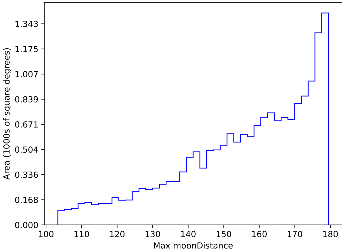
ddf_acor_sf10_lsf15_lsr10_v3.4_10yrs WFD r band: Max moonDistance
