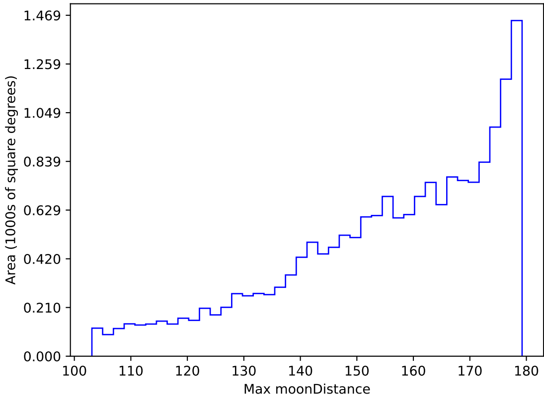
ddf_acor_sf10_lsf15_lsr10_v3.4_10yrs WFD i band: Max moonDistance
