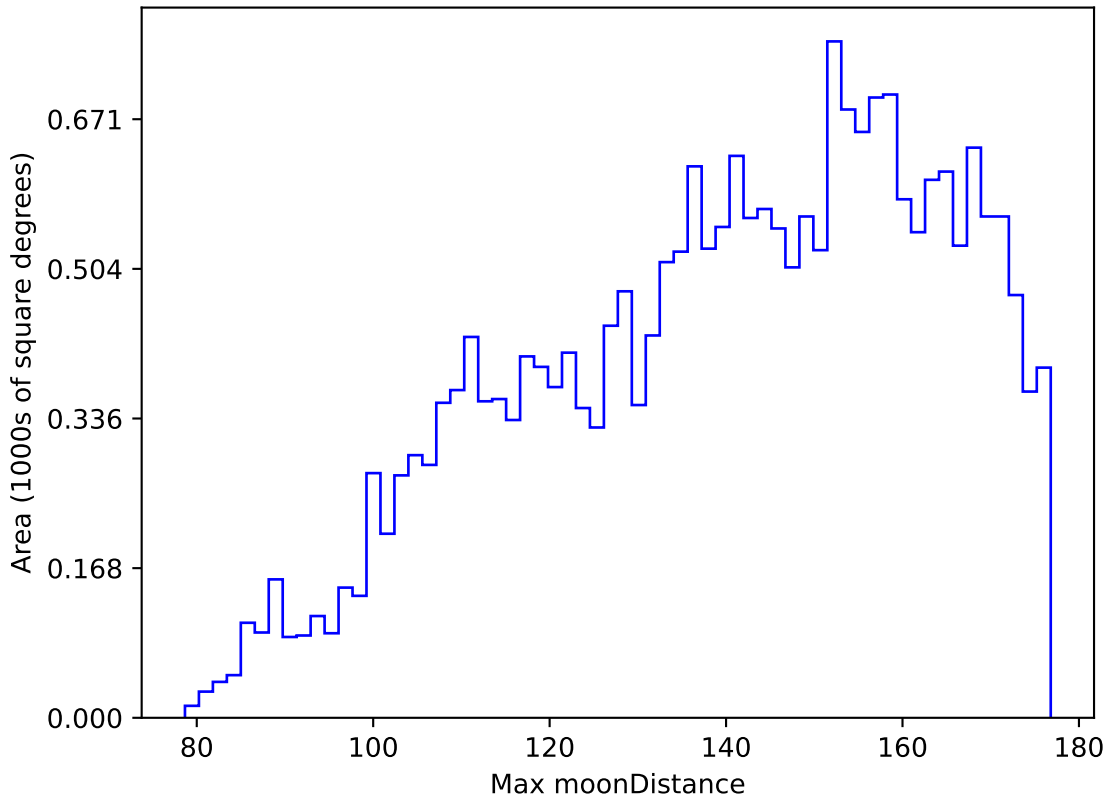
ddf_acor_sf10_lsf15_lsr10_v3.4_10yrs All sky y band: Max moonDistance
