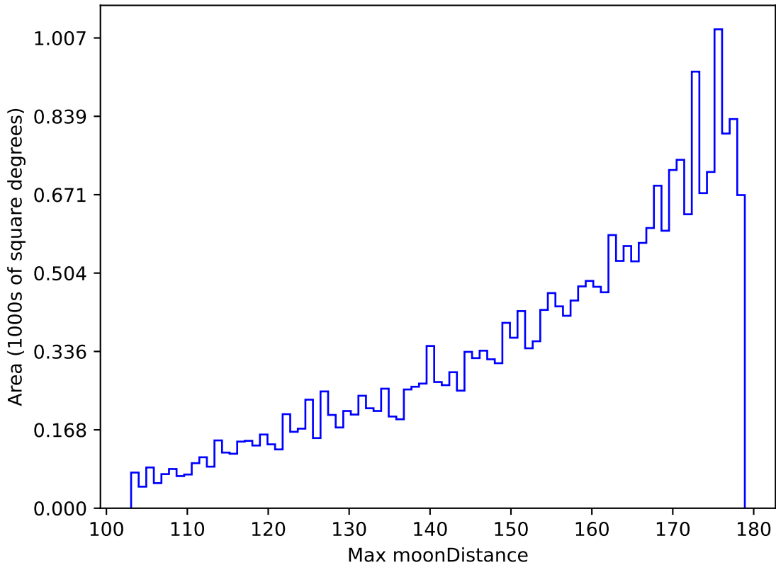
ddf_acor_sf10_lsf15_lsr10_v3.4_10yrs All sky g band: Max moonDistance
