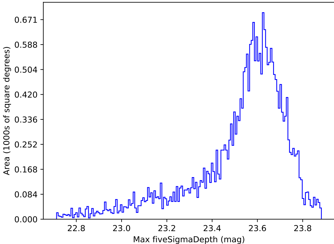
ddf_acor_sf10_ls15_lsr10_v3.4_10yrs All sky z band: Max fiveSigmaDepth
