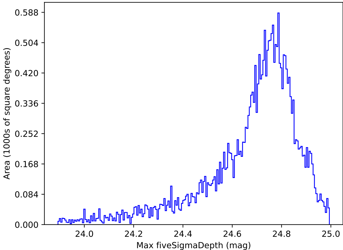
ddf_acor_sf10_ls15_lsr10_v3.4_10yrs All sky r band: Max fiveSigmaDepth
