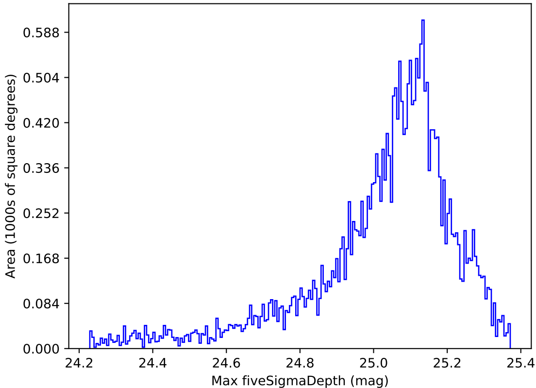
ddf_acor_sf10_ls15_lsr10_v3.4_10yrs All sky g band: Max fiveSigmaDepth
