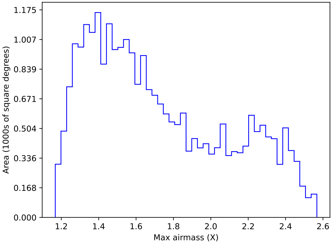
ddf_acor_sf10_ls15_lsr10_v3.4_10yrs Yr 1 r band: Max airmass
