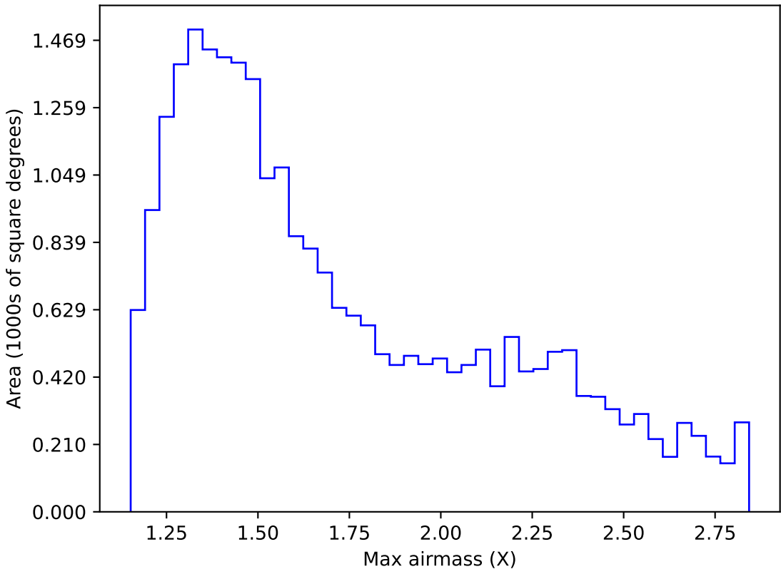
ddf_acor_sf10_lsf15_lsr10_v3.4_10yrs Yr 1 i band: Max airmass
