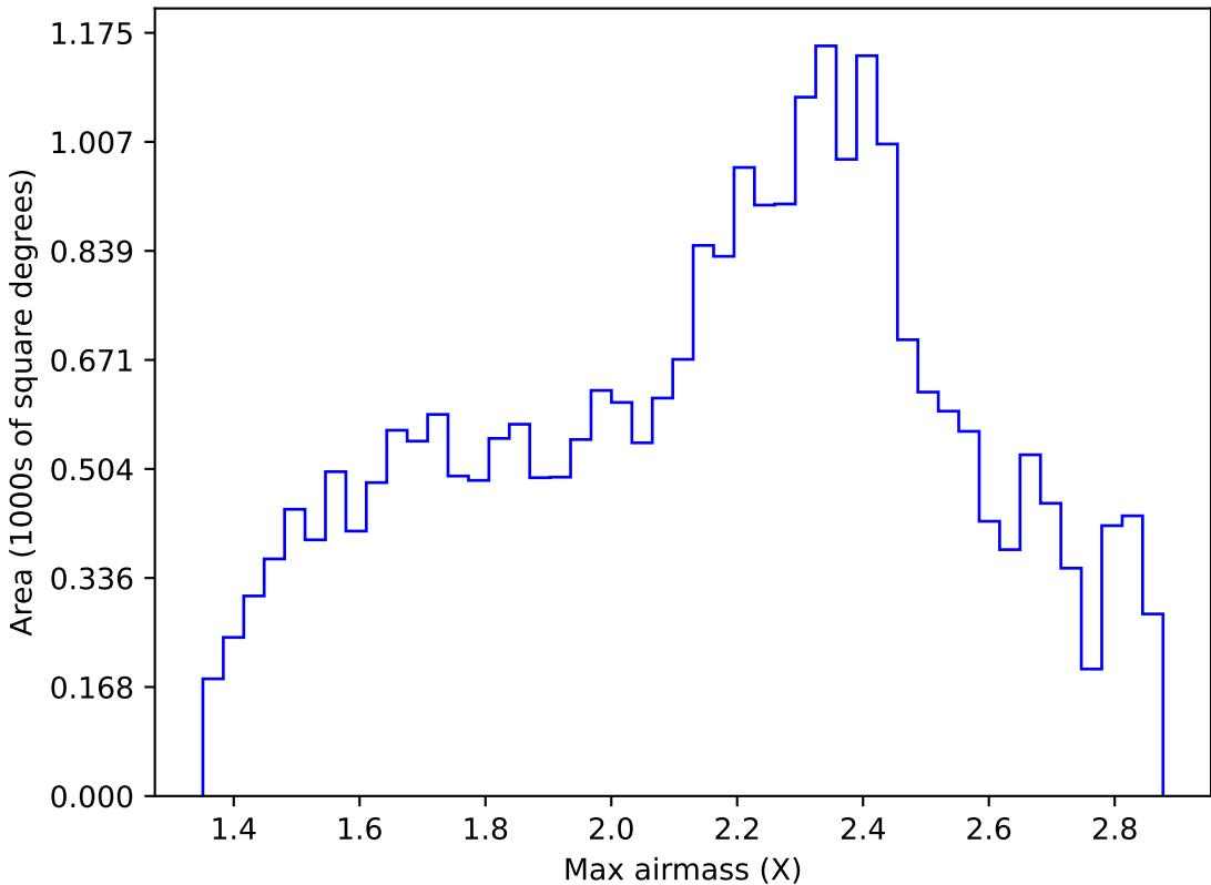
ddf_acor_sf10_lsf15_lsr10_v3.4_10yrs Yr 1 all bands: Max airmass
