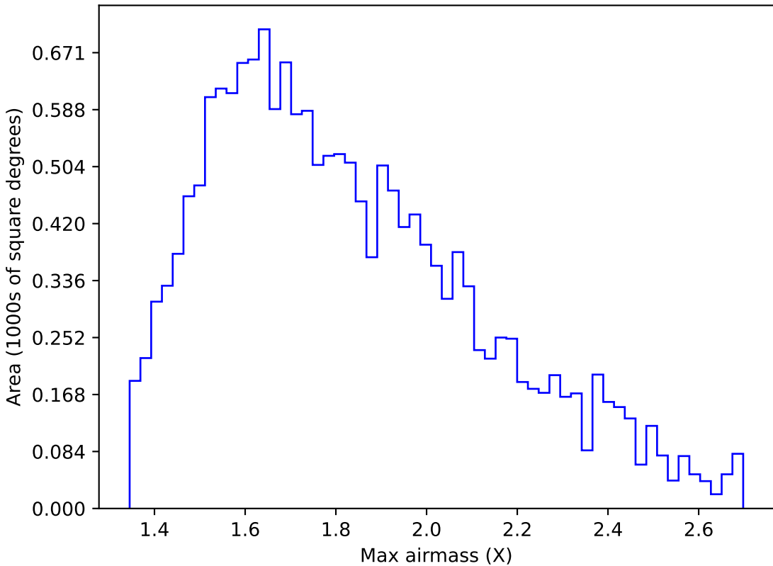
ddf_acor_sf10_lsf15_lsr10_v3.4_10yrs WFD u band: Max airmass
