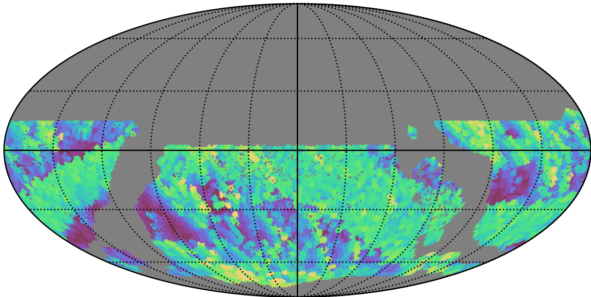
ddf_acor_sf10_lsf15_lsr10_v3.4_10yrs WFD r band: Max airmass
