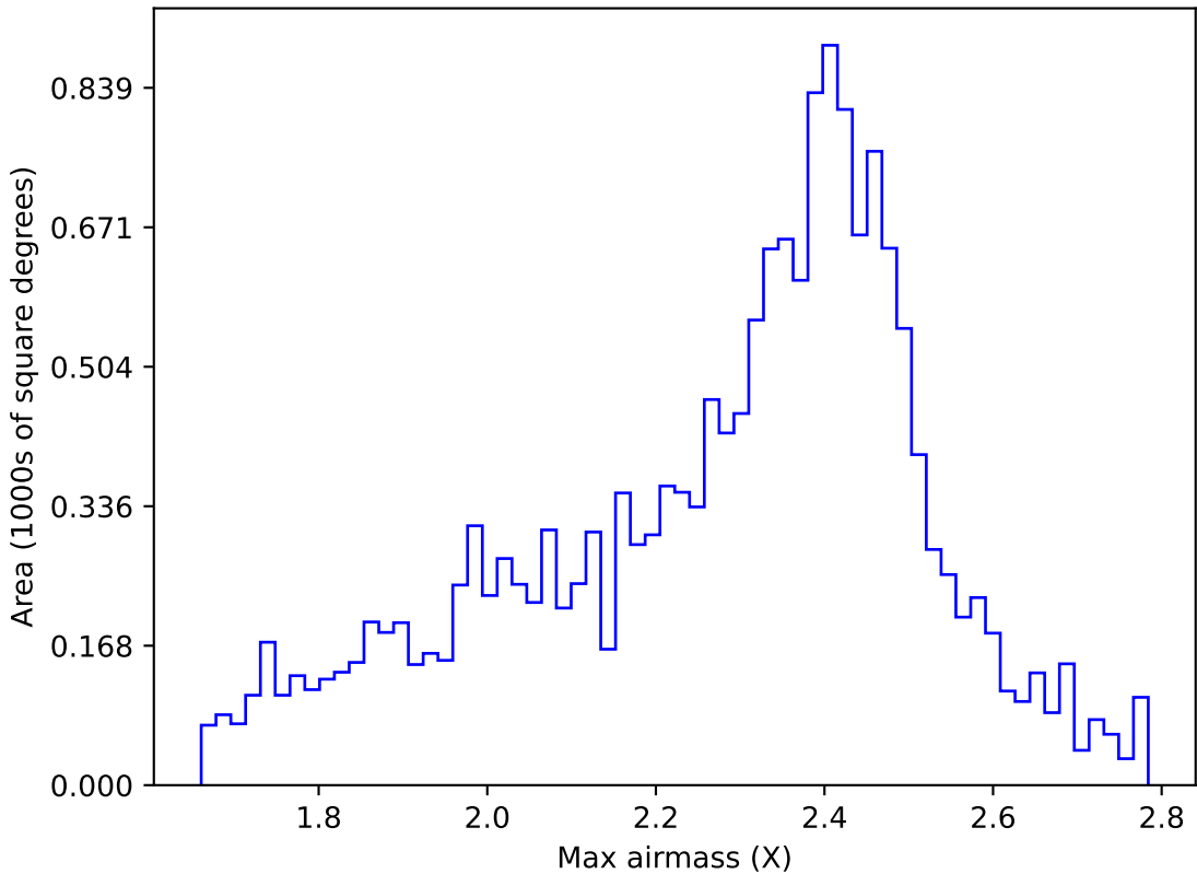
ddf_acor_sf10_lsf15_lsr10_v3.4_10yrs WFD r band: Max airmass
