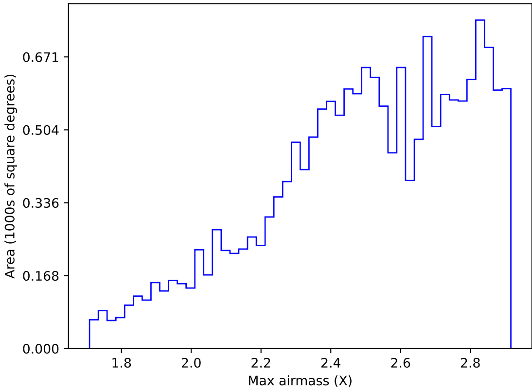
ddf_acor_sf10_lsf15_lsr10_v3.4_10yrs WFD i band: Max airmass
