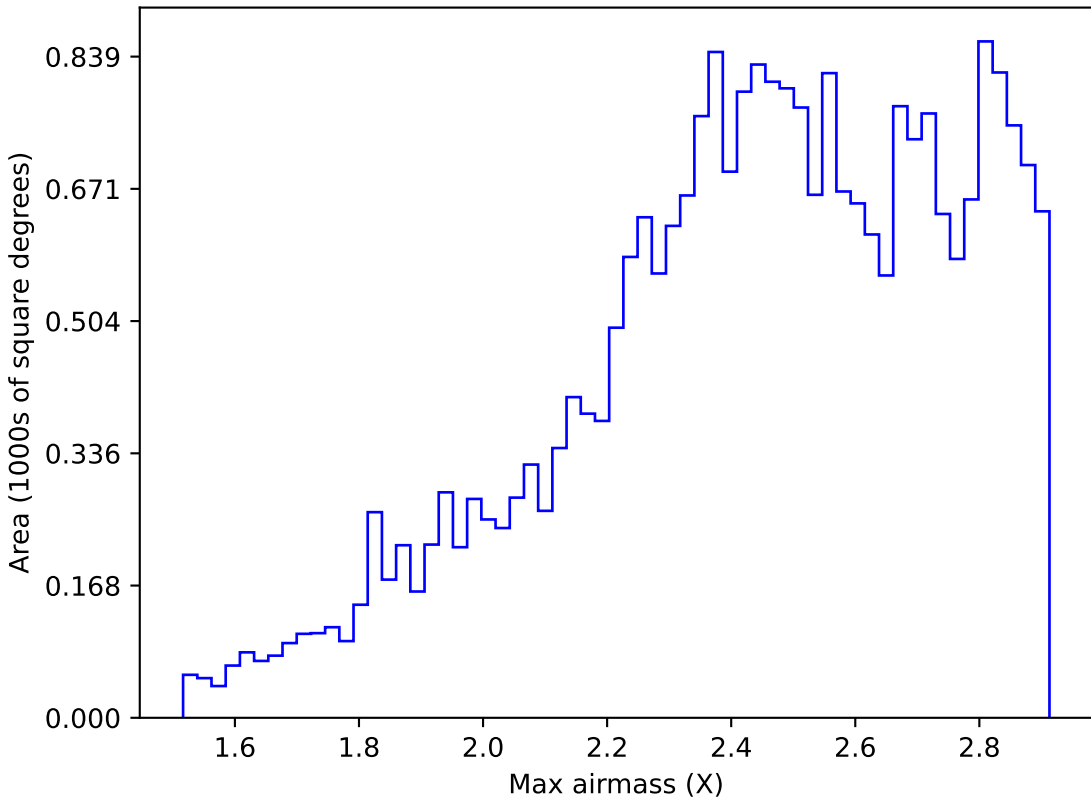
ddf_acor_sf10_lsf15_lsr10_v3.4_10yrs All sky z band: Max airmass
