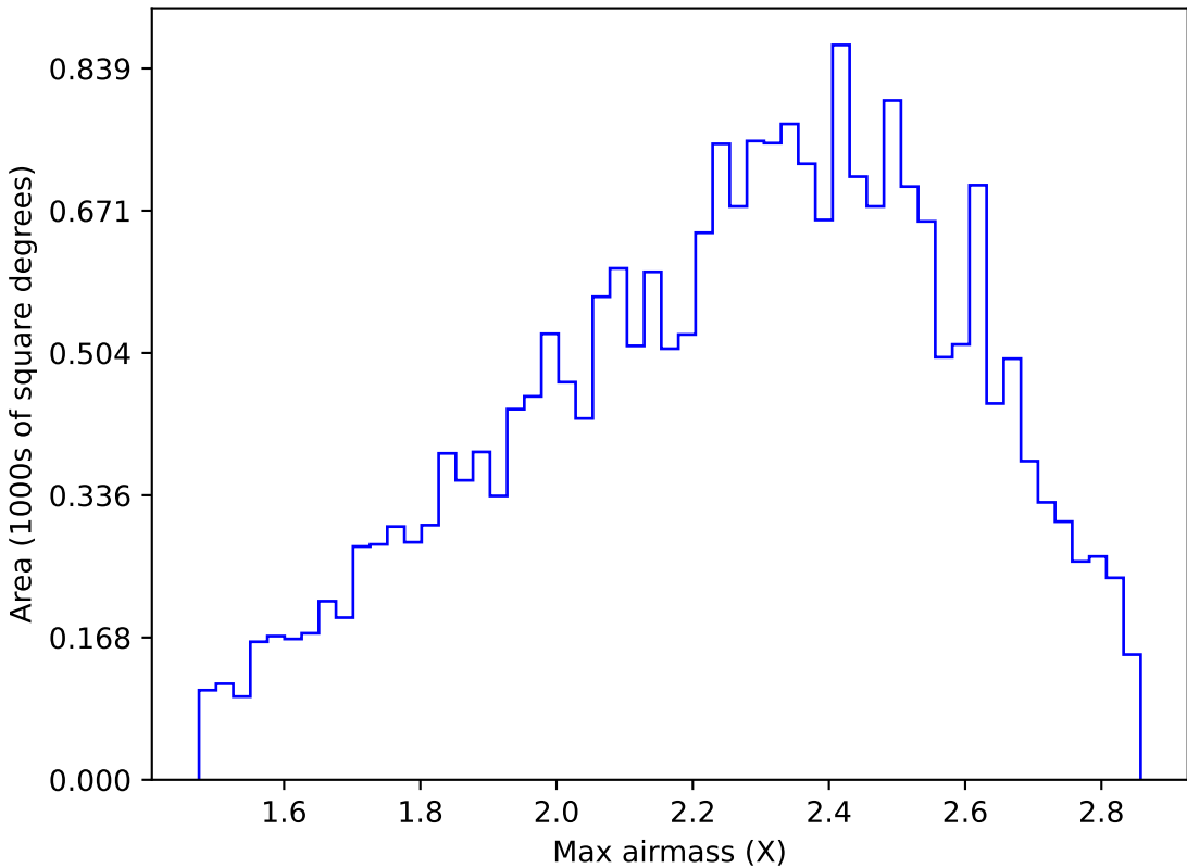
ddf_acor_sf10_lsf15_lsr10_v3.4_10yrs All sky y band: Max airmass
