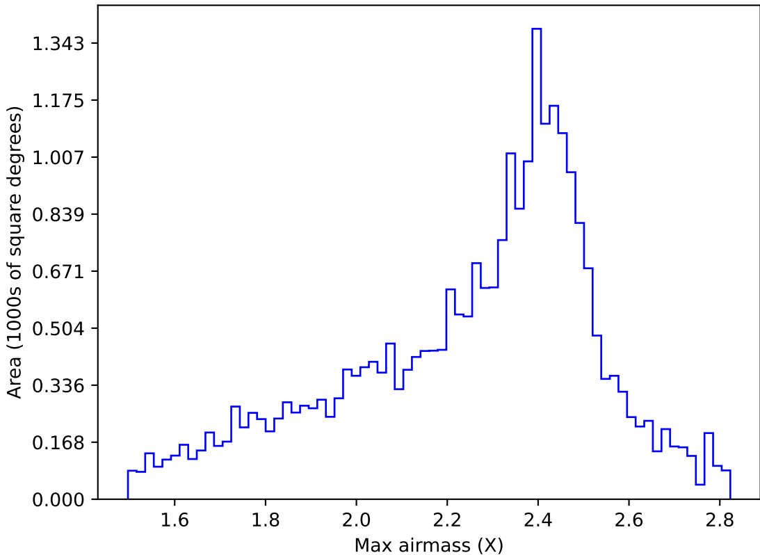
ddf_acor_sf10_lsf15_lsr10_v3.4_10yrs All sky r band: Max airmass
