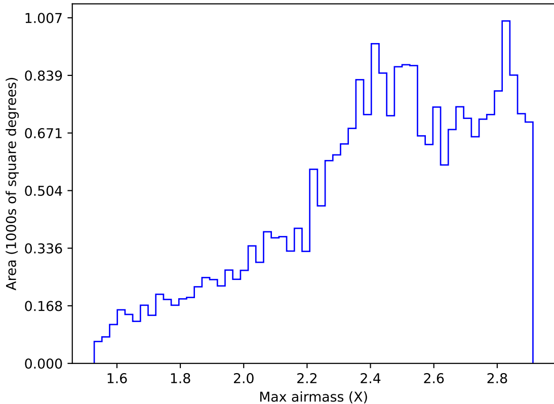
ddf_acor_sf10_lsf15_lsr10_v3.4_10yrs All sky i band: Max airmass
